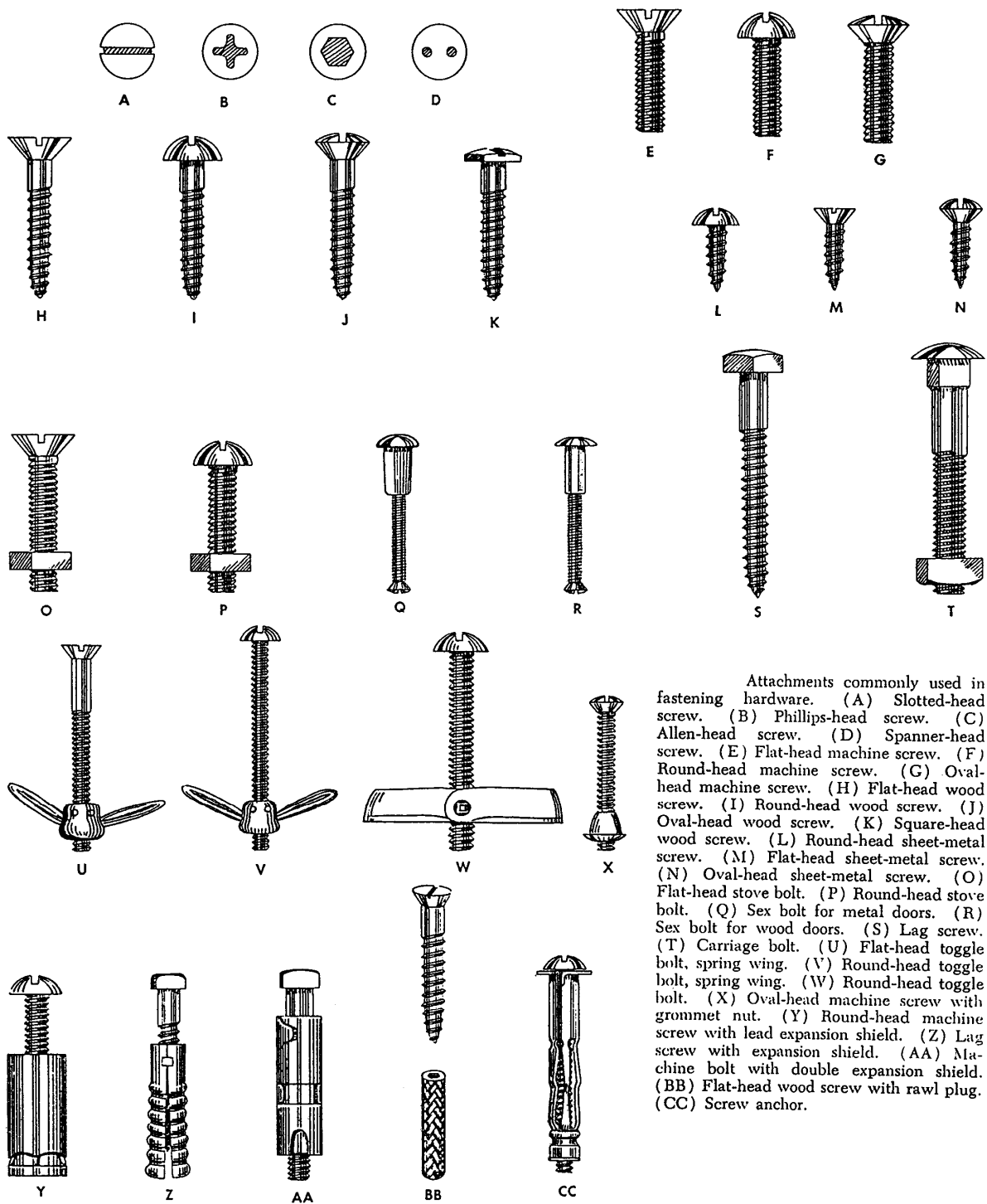
Screw nomenclature from: Brownell, Adon H. n.d. Hardware Age Builders' Hardware Handbook . Chilton Company - Book Division, Philadelphia.
